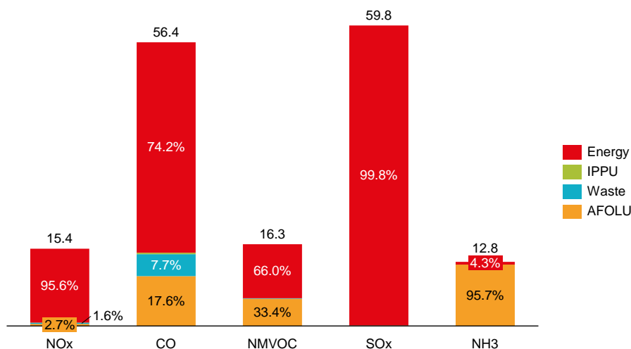
Figure 43. Share of the precursors and indirect GHG emissions by sectors in the year 2014 (in %)
