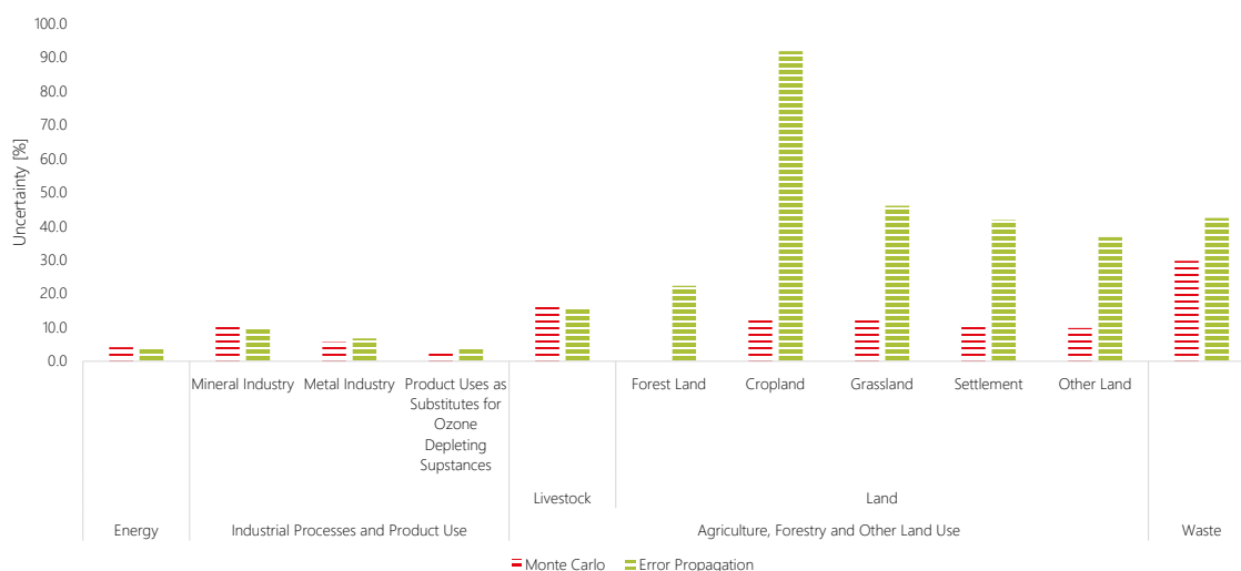
Figure 67. Comparison of Monte Carlo and IPCC Inventory Software method by subcategory for 2014
