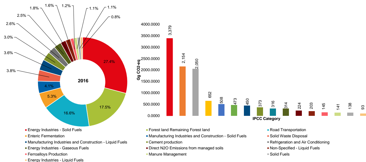
Figure 61. Level assessment of key categories and their contribution in 2016
