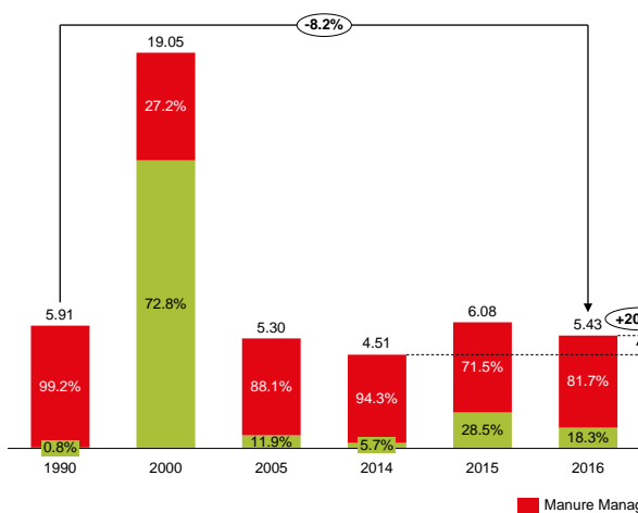
Figure 57. NMVOC emissions from the AFOLU sector, by category (in Gg)
