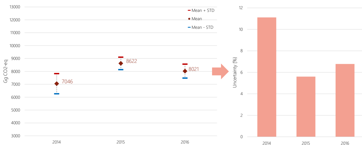
Figure 64. Total yearly emissions (and standard deviation) and total uncertainty for 2014, 2015 and 2016 using Error Propagation method
