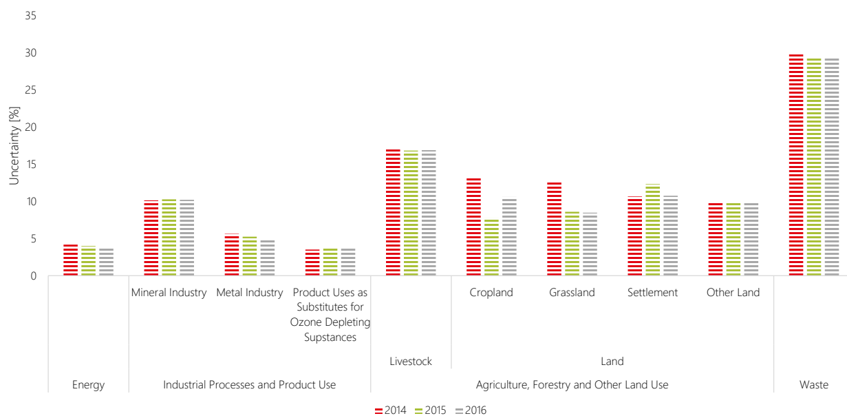
Figure 65. Uncertainty for 2014, 2015 and 2016 using Monte Carlo method by subcategory
