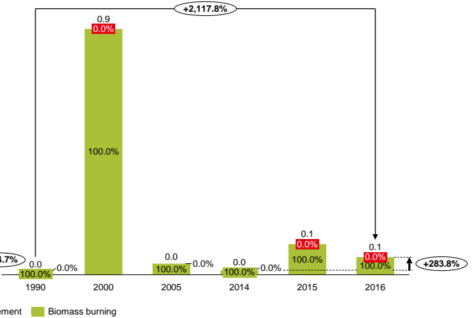
Figure 56. SO 2 emissions from the AFOLU sector, by category (in Gg)
