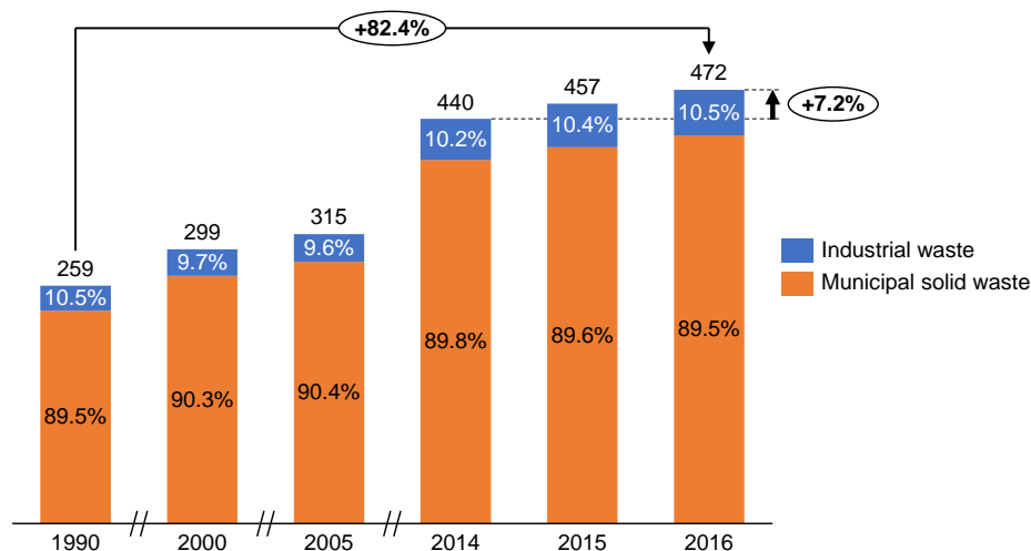
Figure 36. Emissions of CH 4 from Solid Waste Disposal (in Gg CO 2 -eq)
