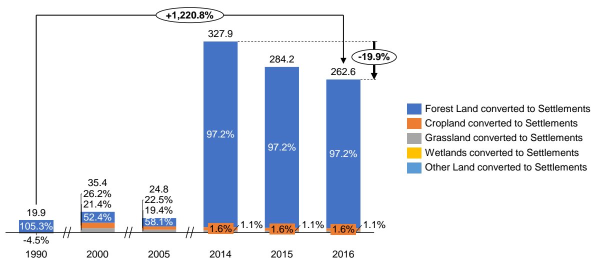
Figure 32. GHG emissions from Other land (in Gg CO 2 -eq)
