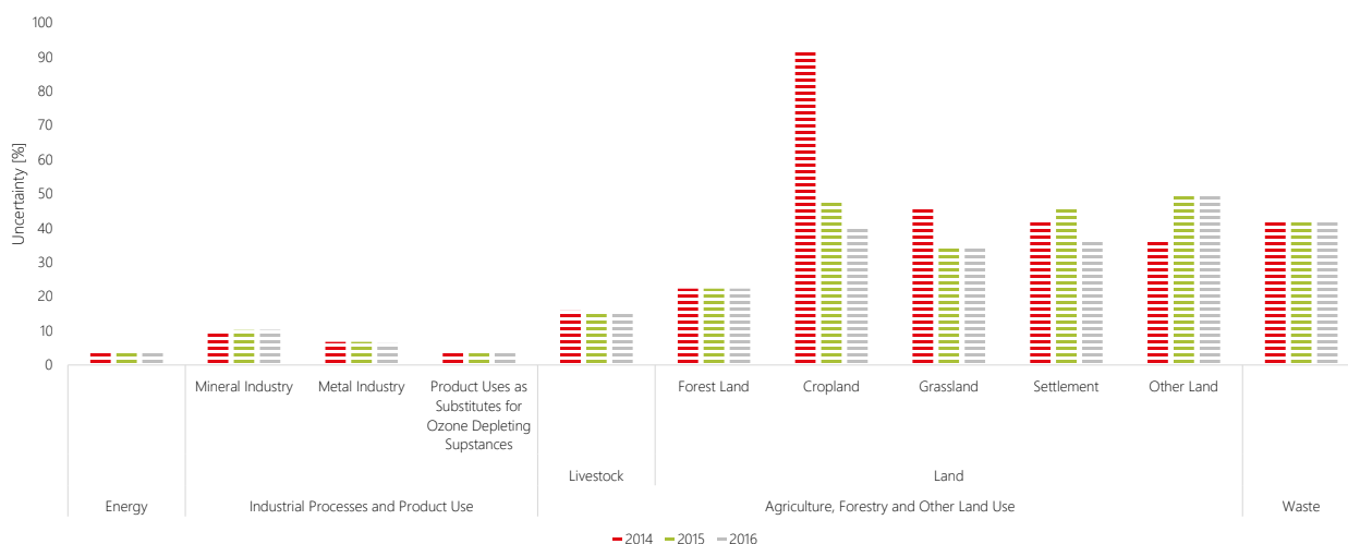
Figure 63. Uncertainty for 2014, 2015 and 2016 using Error Propagation method by subcategory
