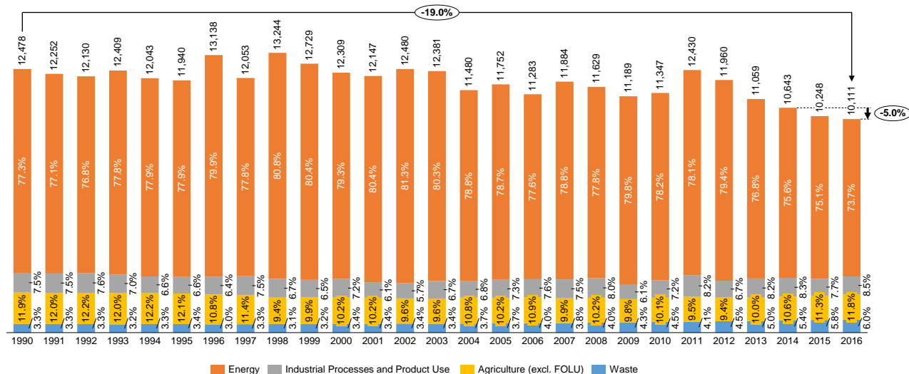
Figure 7. Total GHG emissions by sector, excluding FOLU sector (in Gg CO 2 -eq)
