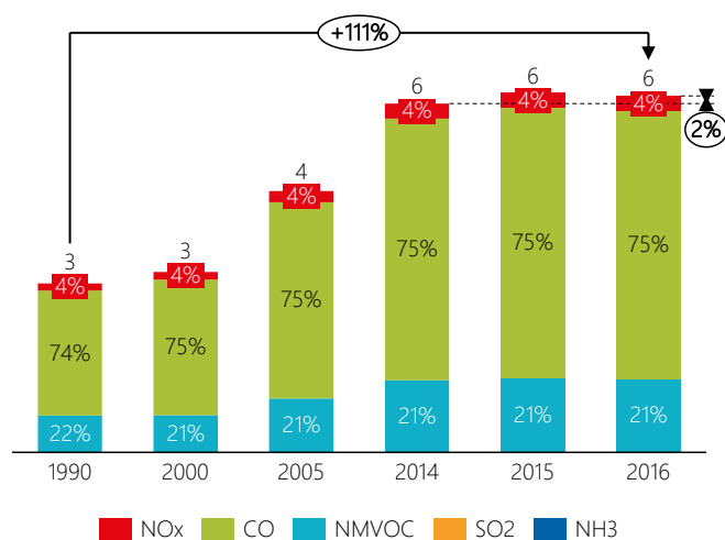
Figure 60. Emissions of NO x , CO, NMVOC and SO 2 from the Waste sector (in Gg)
