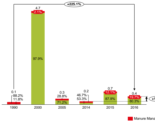
Figure 55. NO x emissions from the AFOLU sector, by category (in Gg)
