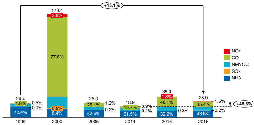
Figure 54. Emissions of NO x , CO, NMVOC, SO 2 and NH 3 from the IPPU sector (in Gg)
