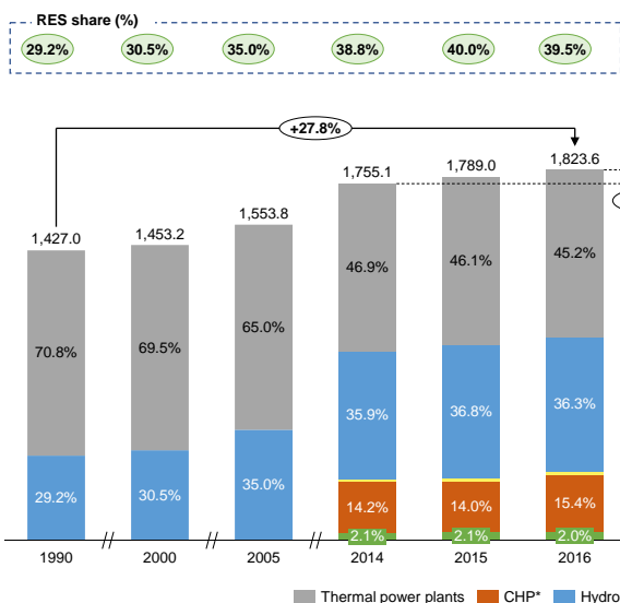
Figure 12. Installed capacity of power plants (only PP that produced electricity in the certain year) (in MW)
